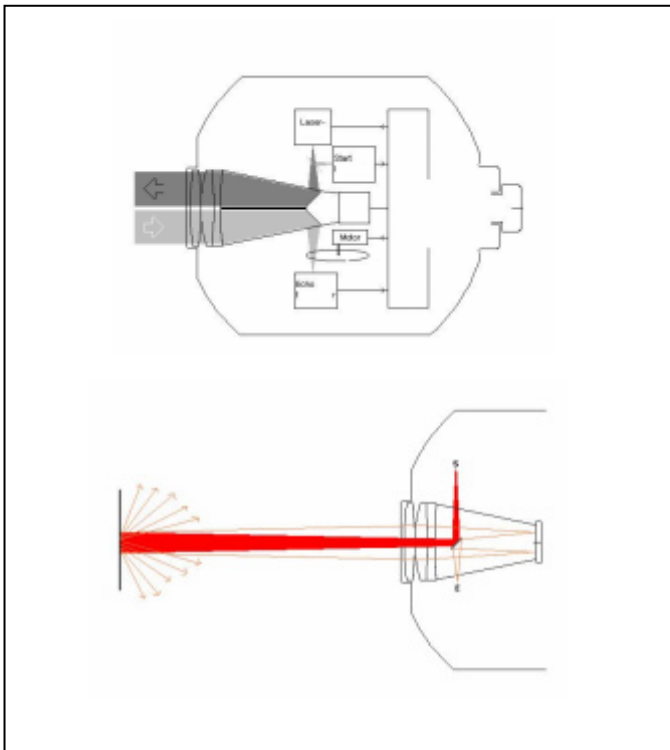
Figure 1: Optical Principles for Pulsed Laser (top) and Phase Shift (bottom) EDM
