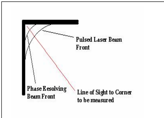
Figure 6: DR Corner Measurement Effect
