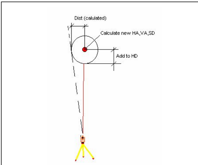
Figure 8: Eccentric Point Measurement
