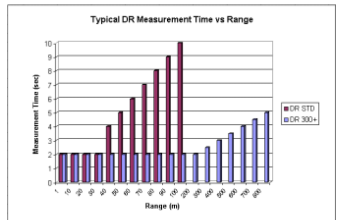
Figure 5: Measurement Time as a Function of Range
